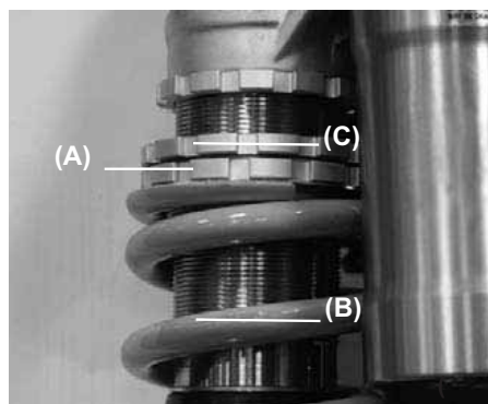
(A) Mutter. (B) Feder. (C) Kontermutter.
