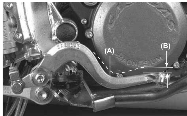
(A). Brake pedal. (B). 10 mm free play.
